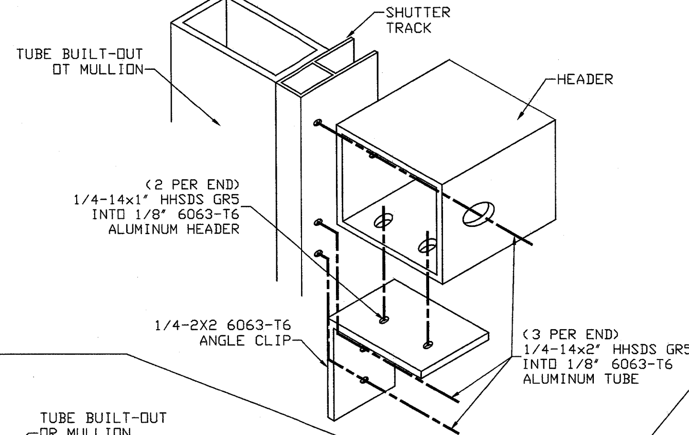
HEADER MOUNT CONNECTION 7
