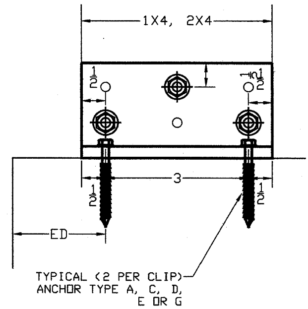
CONNECTION CON 5.3 WITH 2 ANCHORS PER CLIP
