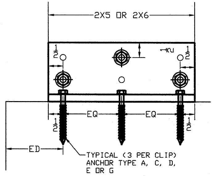
CONNECTION CON 5.4 WITH 3 ANCHORS PER CLIP
